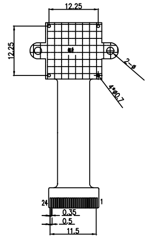
BOTTOM VIEW
